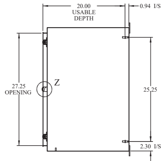
SIDE VIEW (DOOR REMOVED)
