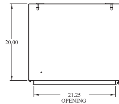
TOP VIEW (DOOR REMOVED)
