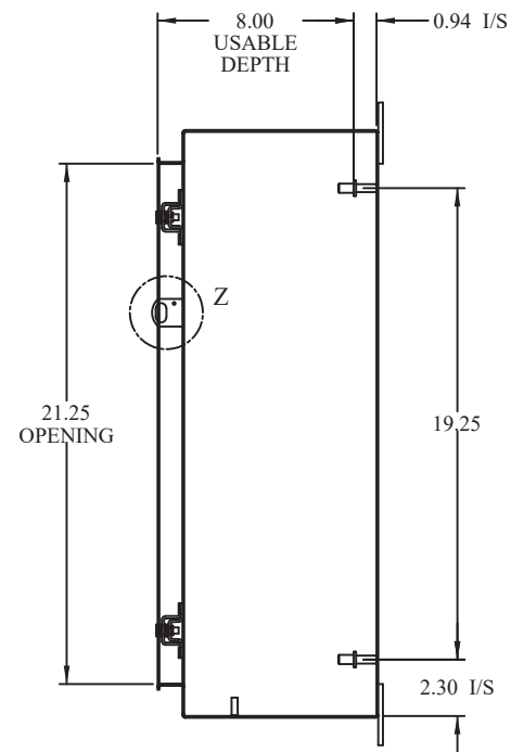
SIDE VIEW (DOOR REMOVED)
