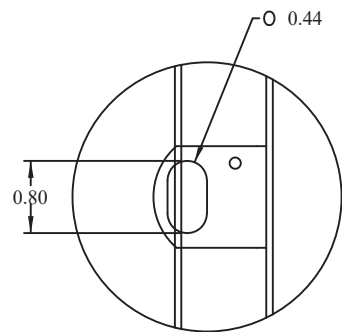
DETAIL Z
