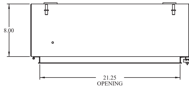
TOP VIEW (DOOR REMOVED)
