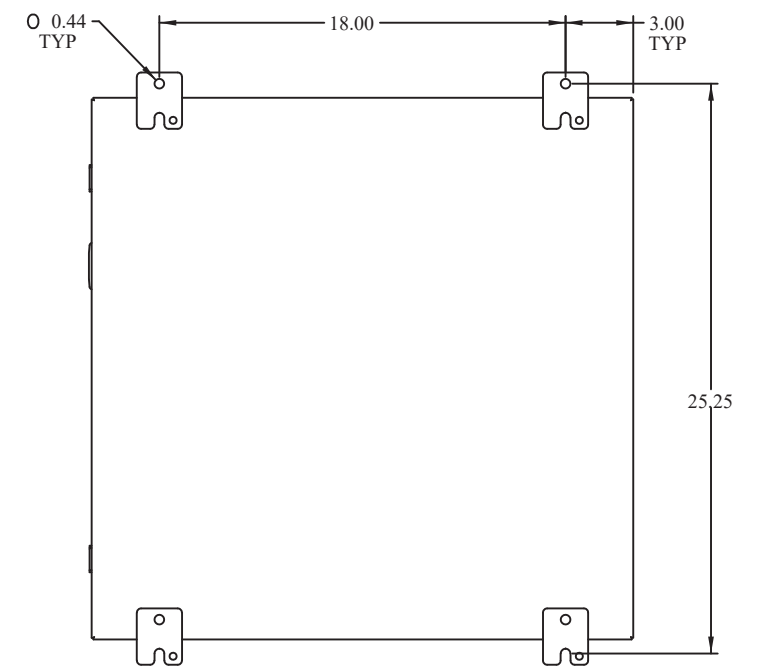
BACK VIEW
