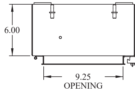
TOP VIEW (DOOR REMOVED)
