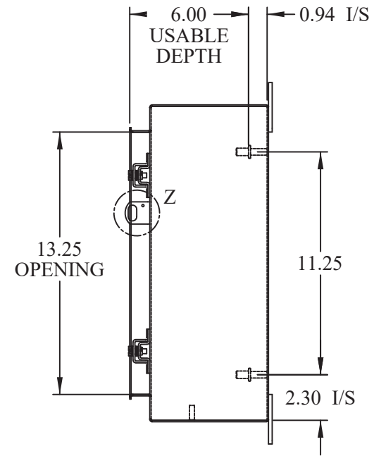
SIDE VIEW (DOOR REMOVED)
