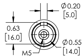
DETAIL A SCALE 2:1
