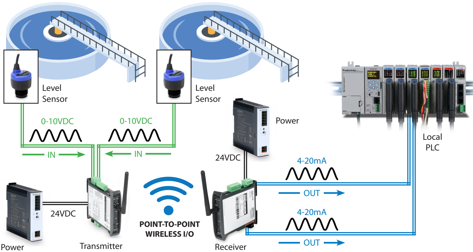
Remote Water Tank #1
