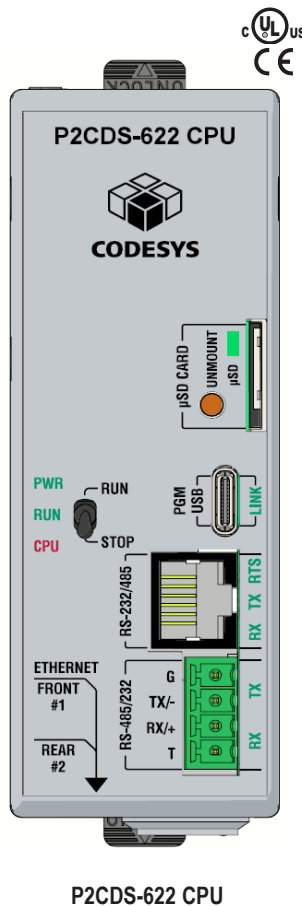
P2CDS-622 CPU
