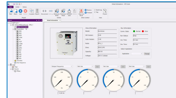
VFD Suite allows you to see everything there is to know about the connected drive
