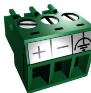
DC Power Connector Part No. EA-MG-DC-CON
