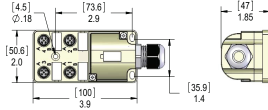
Figure 2: 4-Port, 5-Wire/5-Pole
