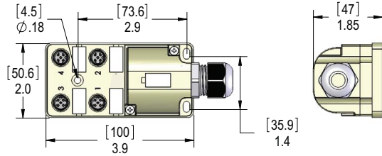
Figure 1: 4-Port, 4-Wire/5-Pole
