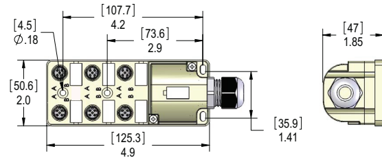
Figure 4: 6-Port, 5-Wire/5-Pole
