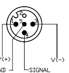
No LED Version Diagram 5-A
