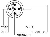
No LED Version Diagram 6-A
