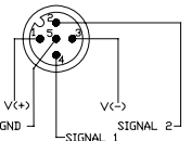
No LED Version Diagram 4-A
