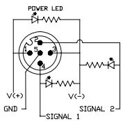
PNP Version Diagram 6-B
