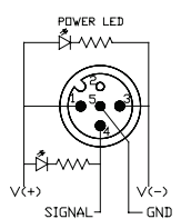
NPN Version Diagram 5-C
