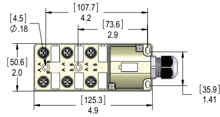
Figure 4: 6-Port, 5-Wire/5-Pole
