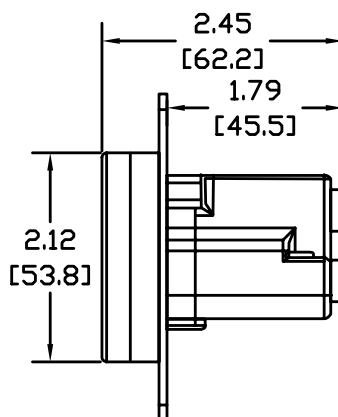
6x32 TAP 1.81 [46.0] 3.28 [83.3] 2.37 [60.2] 3.68 [93.5] 2.50 [63.5] 2.25 [57.2]
