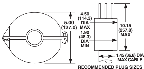
RECOMMENDED PLUG SIZES
