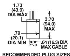
RECOMMENDED PLUG SIZES
