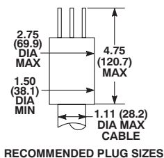
RECOMMENDED PLUG SIZES
