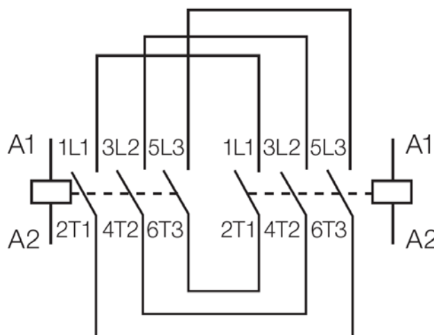
Electric Diagram
