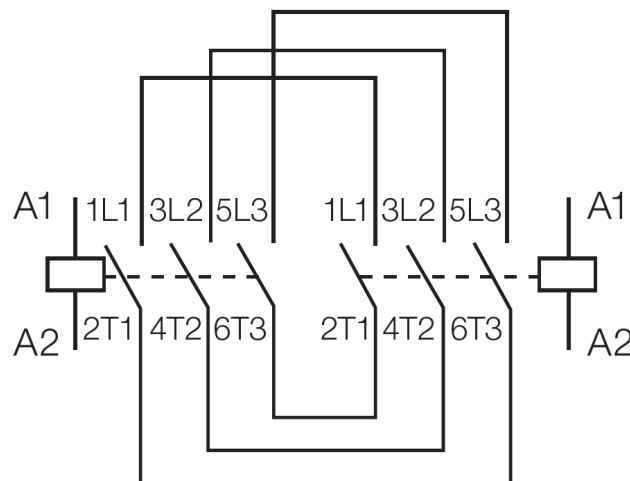
Electric Diagram
