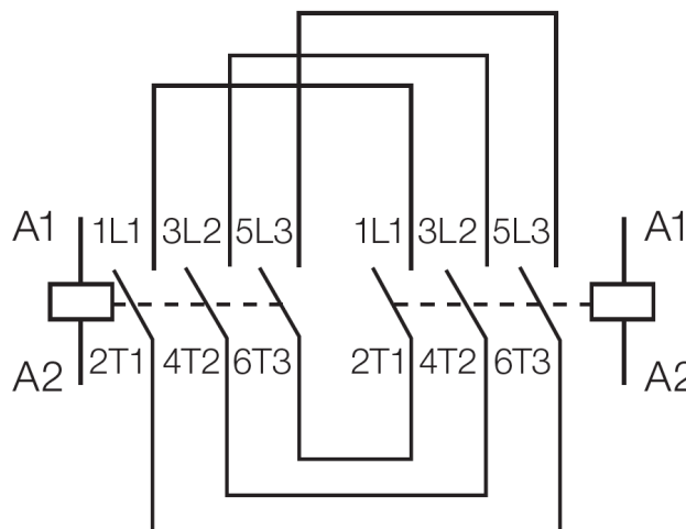
Electric Diagram
