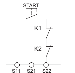
Contactor Manual Feedback
