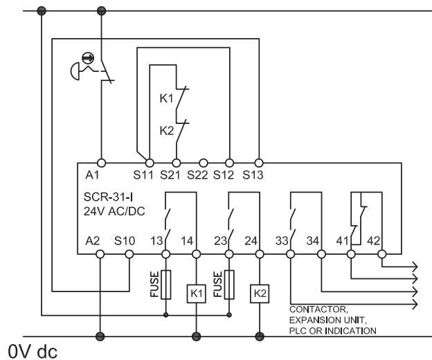
Automatic restart mode (single channel) non contact
