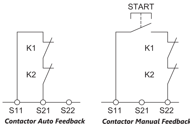
Contactor Auto Feedback
