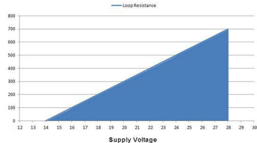
Maximum Loop Resistance in \Omega
