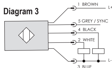
Connector M12 connector
