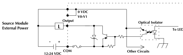
Equivalent Output Circuit
