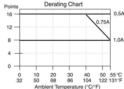
T1K-16TD2-1 Derating Chart
