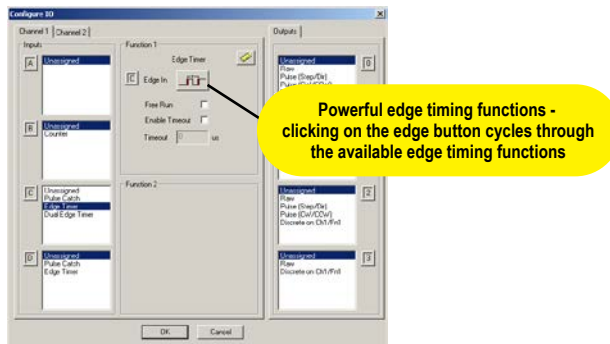
Using Configure I/O screen to configure CTRIO for high-speed timing
