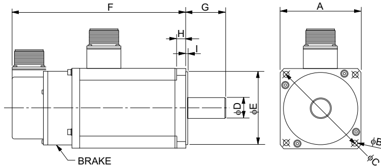
SureServo® Motor Dimensions -1000W Low Inertia
