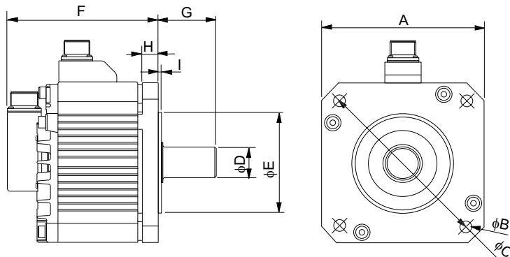
SureServo® Motor Dimensions -1000W-3000W Medium Inertia
