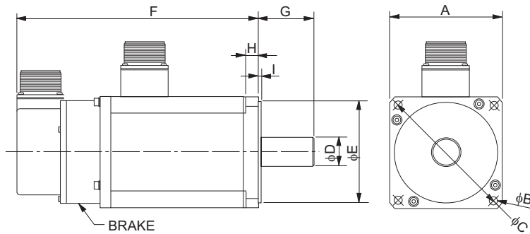
SureServo® Motor Dimensions -1000W Low Inertia
