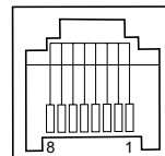
8 pin RJ45
