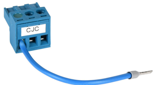
External reference junction (CJC) is required for thermocouple applications with 9182-10-51-11S
