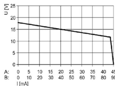
Output characteristic 9175-20-14-11, 9176-20-14-00
