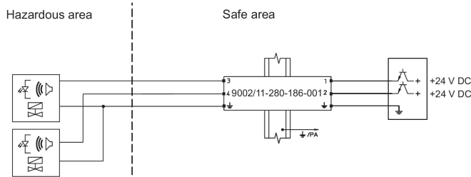
Application: Discrete 2-wire output for solenoid valves, LEDs and signalling devices
