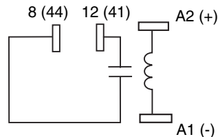
Figure 2 AD-70S2-xx wiring diagram
