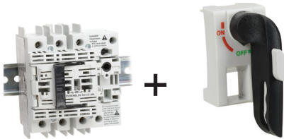
Direct Operation
