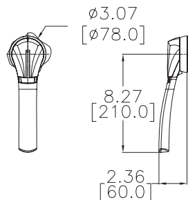
Handle Dimensions
