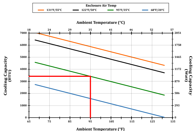
SCE-AC3400 Units
