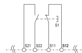
Fct.: Exclusive XOR contacts (5), with cross fault detection SIL 3, PL e, Cat. 4
