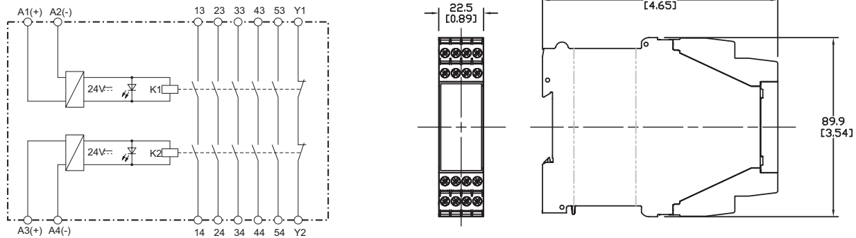
LG5929 Block Diagram
