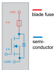
Schematic diagram REX-T
