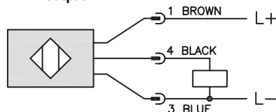
Diagram 1 PNP Output
