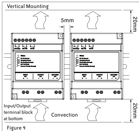
RHINO PSL-24-BCM240 Battery Control Module
