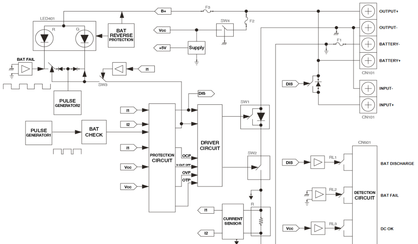
RHINO PSL-24-BCM240 Battery Control Module
