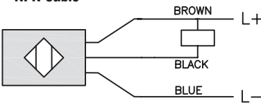
NPN Cable
