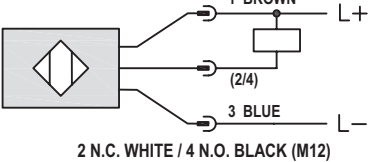
NPN Connector
