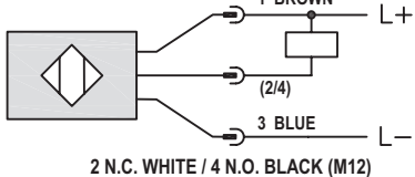
NPN Connector
