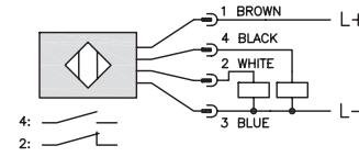
Diagram 4 PNP Output
