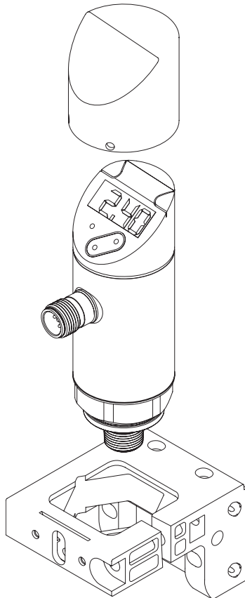
Assembly Example
