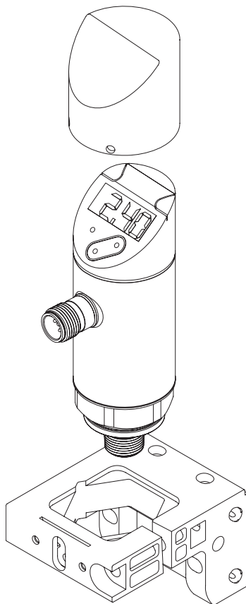
Assembly Example
