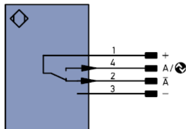
Diagram 1 PNP
