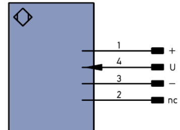
Diagram 3 Emitter
