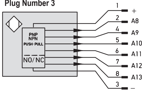
Plug Number 3
