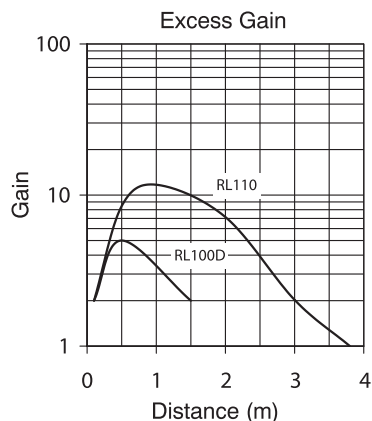
Chart 3 (Throughbeam)
