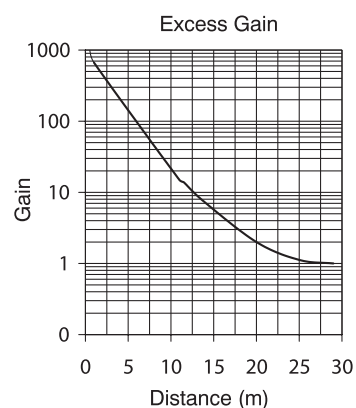
Chart 3 (Throughbeam)
