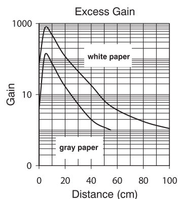
Chart 2 (Polarized Reflective)
