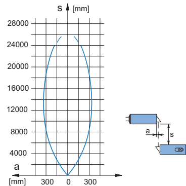
Chart 8 (Through-beam C18R-*-2*)
