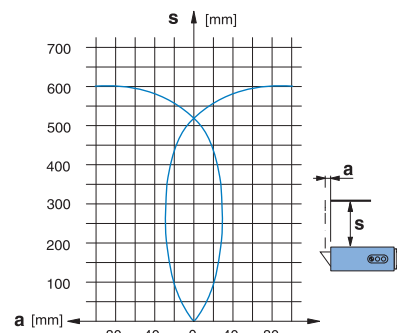
Chart 6 (Diffuse c18D-*-2*)
