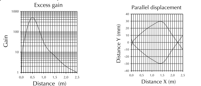
Chart 4 (Through-beam)
