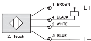
Diagram 1 NPN Output
