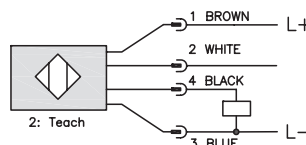
Diagram 2 PNP Output
