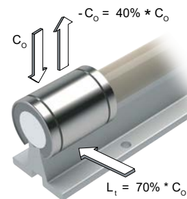
Open Bearing
