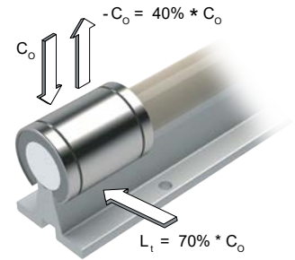
Open Bearing
